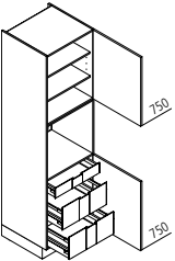
GBI Appliance housing for oven / microwave ↔ 60 ↑ 195/210/225 ↩ 60
