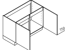
SOD Sink base unit ↔ 80/90/100/120 ↑ 75 ↙ 60
