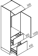
GKZ Appliance housing for refrigerator / recess 1025mm
