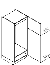
GKG Appliance housing for fridge/ freezer combination / recess 1225 mm
