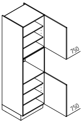
GB Appliance housing for oven / microwave ↔ 60 ↑ 195/210/225 ↩ 60
