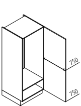
GK Appliance housing for refrigerator / recess 1225mm
