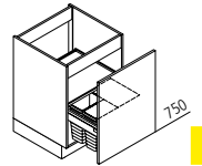
SABHD Sink base unit with hanging waste separation system ↔ 40/45/60 ↑ 75 ↙ 60
