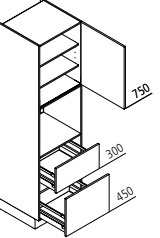
GBZ Appliance housing for oven / microwave ↔ 60 ↑ 195/210/225 ↩ 60
