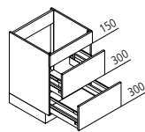
SAK Sink base unit ↔ 60/80/90/100/120 ↑ 75 ↙ 60
