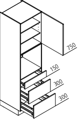
GBAK Appliance housing for oven / microwave ↔ 60 ↑ 195/210/225 ↩ 60
