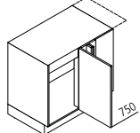
UESAD Space filler for corner sink base unit ↔ 110/115/125 ↑ 75 ↙ 60
