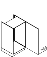
GK Appliance housing for refrigerator / recess 1025mm
