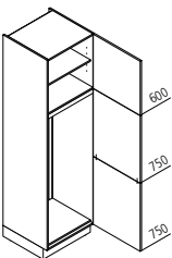
GK Appliance housing for refrigerator / recess 1440mm
