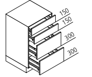
USA Drawer base unit ↔ 30/40/45/50/60/80/90/100/120 ↑ 90 ↙ 60/35
