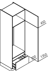
GKA Appliance housing for refrigerator / recess 1225mm
