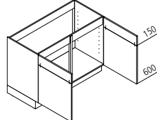
SO Sink base unit ↔ 80/90/100/120 ↑ 75 ↙ 60
