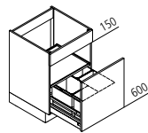
SAB Sink base unit ↔ 45/50/60 ↑ 75 ↙ 60
