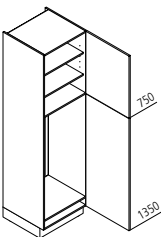
GK Appliance housing for refrigerator / recess 1225mm
