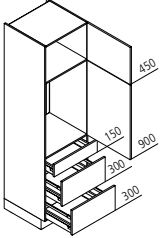
GKAK Appliance housing for refrigerator / recess 880mm
