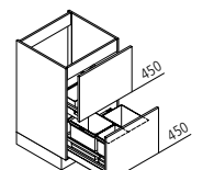
SUZ SSink base unit ↔ 60/80/90/100/120 ↑ 90 ↙ 60
