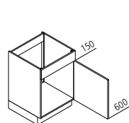
SO Sink base unit ↔ 45/50/60 ↑ 75 ↙ 60
