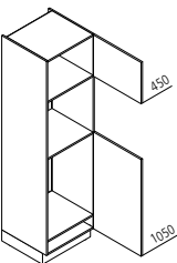
GKB Appliance housing for refrigerator and oven / recess 880 mm
