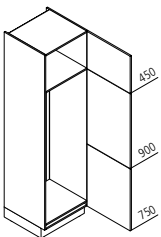
GKG Appliance housing for fridge/freezer combination / recess 1580 mm
