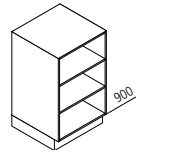
UR Base unit ↔ 15/20/25/30/35/40/45/50/55/60 ↑ 90 ↙ 60/35
