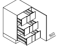
UIADD Base unit ↔ 40/45/50/60 ↑ 90 ↙ 60/35
