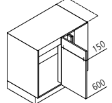
UESA Space filler for corner sink base unit ↔ 110/115/125 ↑ 75 ↙ 60
