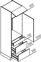
GKAK Appliance housing for refrigerator / recess 1025mm
