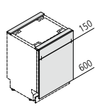
GSBS Front panel for fully integrated dishwasher ↔ 45/60 ↑ 75 ↙ 60
