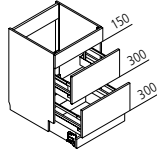
SABS Sink base unit with large-capacity pull-out drawer ↔ 60/80/90/100 ↑ 75 ↙ 60
