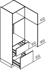
GKZ Appliance housing for refrigerator / recess 880mm
