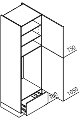
GKA Appliance housing for refrigerator / recess 1025mm
