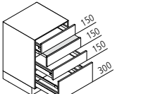
USAP Drawer base unit with work table
