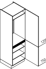
GK Appliance housing for refrigerator / recess 1025mm
