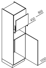
GKL Appliance housing with lift-up door for refrigerator / microwave / recess 1025 mm ↔ 60 ↑ 195/210/225 ↩ 60
