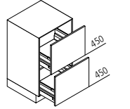
UZ Pull-out unit ↔ 30/40/45/50/60/80/90/100/120 ↑ 90 ↙ 60/35
